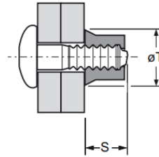
Full Collar
