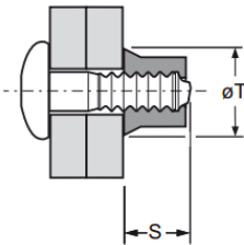
Full Collar
