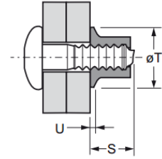
Flanged Collar
