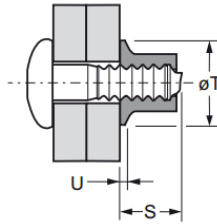
Flanged Collar
